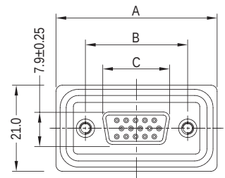
Female DSub
