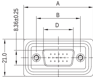
Male DSub
