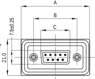
Female DSub
