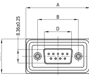
Male DSub
