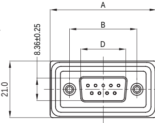
Male DSub
