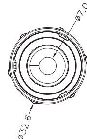
Clamp Ring
