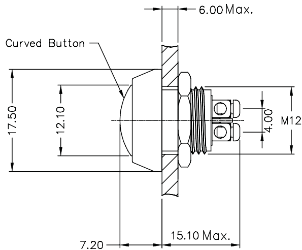
Quick Connect
